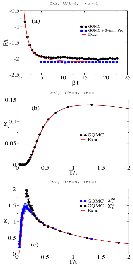
FIG. 1: a) Energy as a function of inverse temperature as obtained from exact diagonalization (solid line), from the GQMC (bullets) and from the GQMC supplemented by the symmetry projection (squares). Here we have projected onto the total spin s = 0 state and d -wave lattice symmetry. (b) The charge susceptibility and (c) the longitudinal and transverse spin susceptibilities. In the above, we use 60'000 walkers, an imaginary time step of \Delta\tau t = 0.0001 , an explicit Euler scheme with adaptive time step, and \sigma = \sigma^z in Eq. (1)
