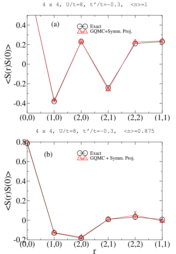
FIG. 3: Real space spin-spin correlations as obtained from the GQMC and comparison with exact-diagonalization results. See caption of Table III for details of the GQMC simulations.
