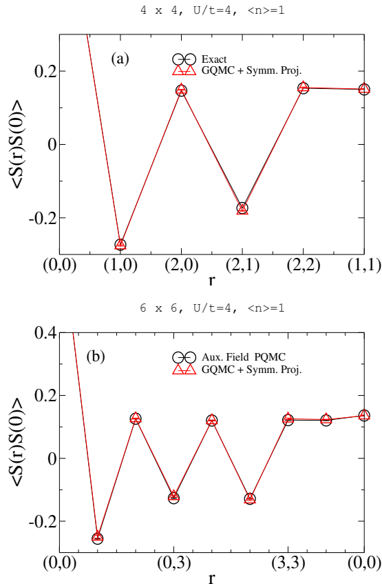
FIG. 2: Real space spin-spin correlations as obtained from the GQMC and comparison with benchmark results. See caption of Table II for details of the GQMC simulations.
