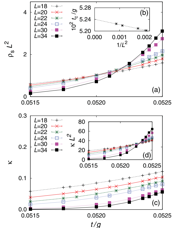
FIG. 4. (Color online) Scaling of the superfluid density \rho_s and compressibility \kappa across the fixed-density transition at \mu/g = 0.185 [12] using \beta g = L^2/4 . In (a), the intersect of curves for consecutive system sizes [shown in (b)] approaches the t_c obtained in Figs. 2 and 3. (c) Shows the compressibility for the same parameters, with no intersection in the vicinity of t_c . (d) Illustrates the intersect obtained when plotting \kappa L^2 .
