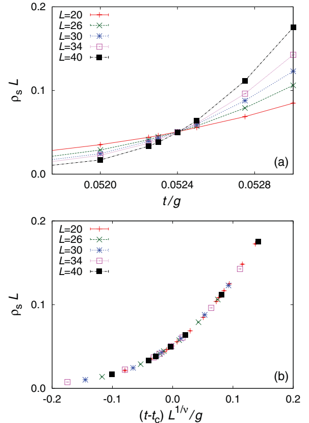
FIG. 2. (Color online) Scaling of the superfluid density \rho_s across the fixed-density transition at \mu/g = 0.185 [12] using L \times L square lattices and \beta g = 2L . The intersect of L \rho_s for different lattice sizes L in a single point in (a) is evidence for a dynamical critical exponent z = 1 , and defines the critical point at t_c/g = 0.05242(1) . (b) Scaling collapse using t_c/g = 0.05242 and \nu = 0.6715 [4].
